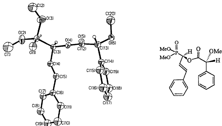
Figure 1: The molecular structure (projection plot) of O-methyl mandelate 4b shown with 50% probability ellipsoids. Due to the lack of observed reflections, positional and isotropic thermal parameters were refined for the hydrogens atoms on the asymmetric carbon atoms, C3 [C(1)] and C13 [C(2')].
